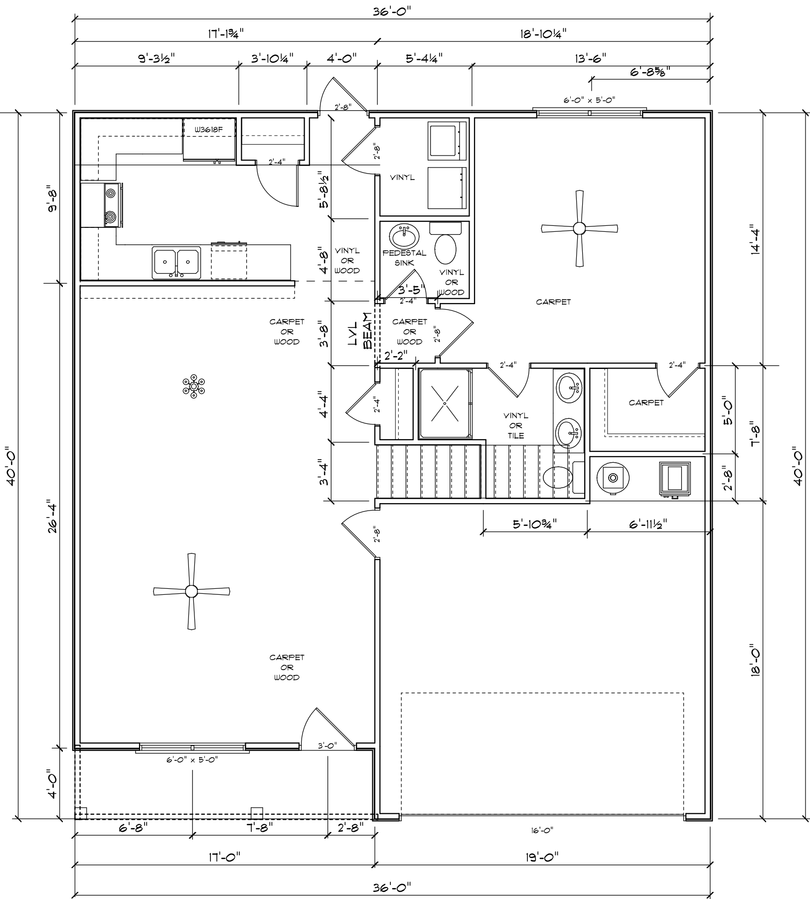
1667 AMHURST MODEL - MAIN FLOOR
