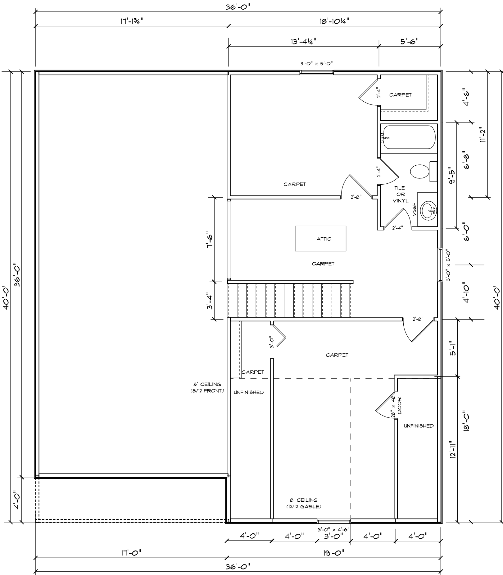
1667 AMHURST MODEL - TOP FLOOR
