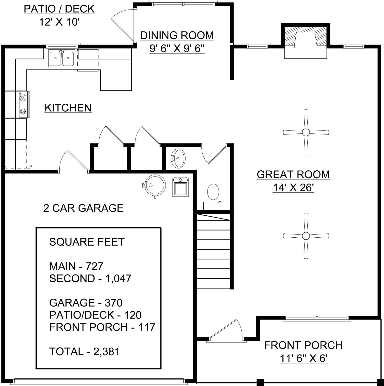
RIDGEWOOD 3 BR MODEL - FIRST FLOOR - LUTTRELL DEVELOPMENT
