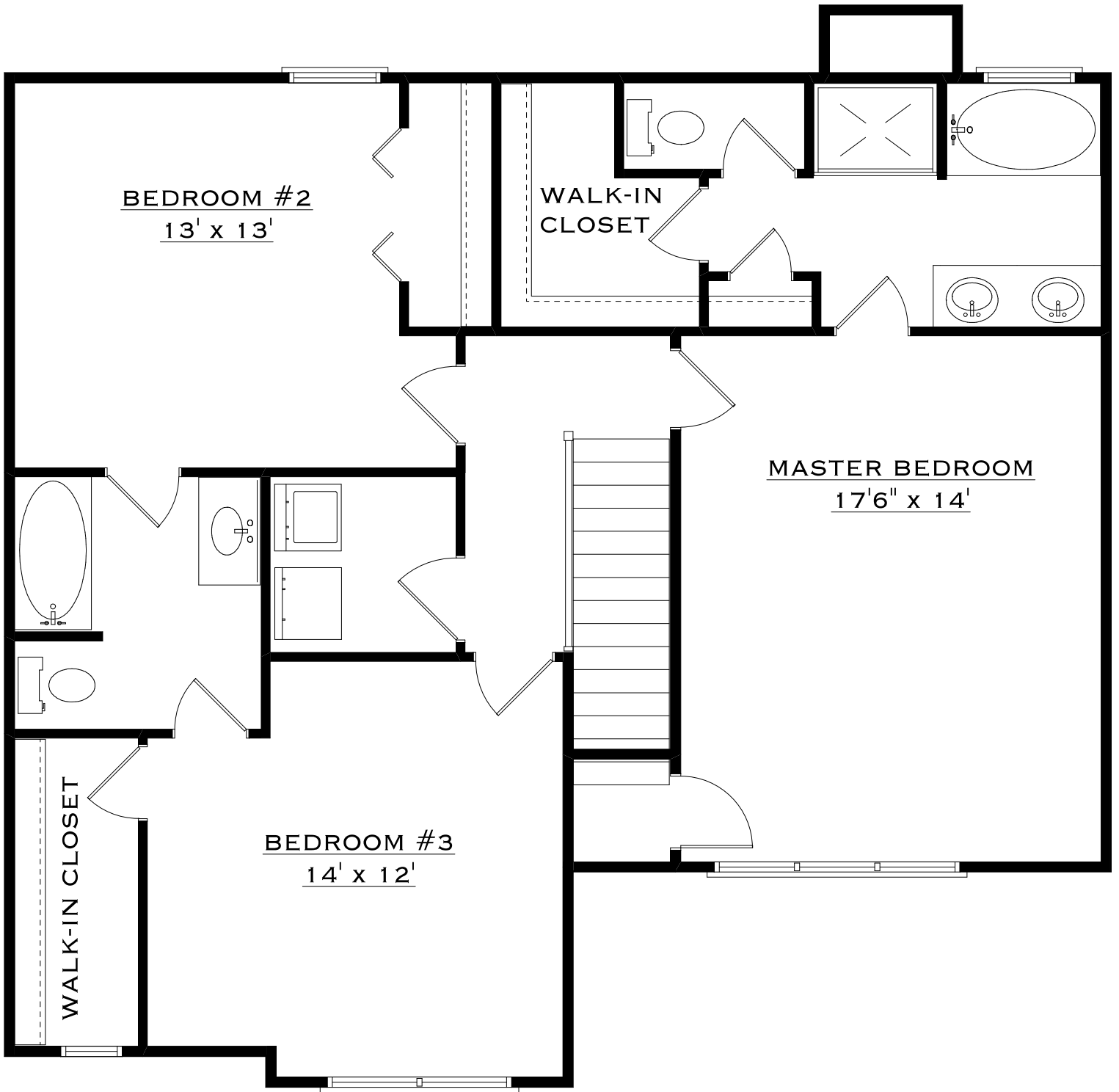
RIDGEWOOD 3BR MODEL - SECOND FLOOR - LUTTRELL DEVELOPMENT
