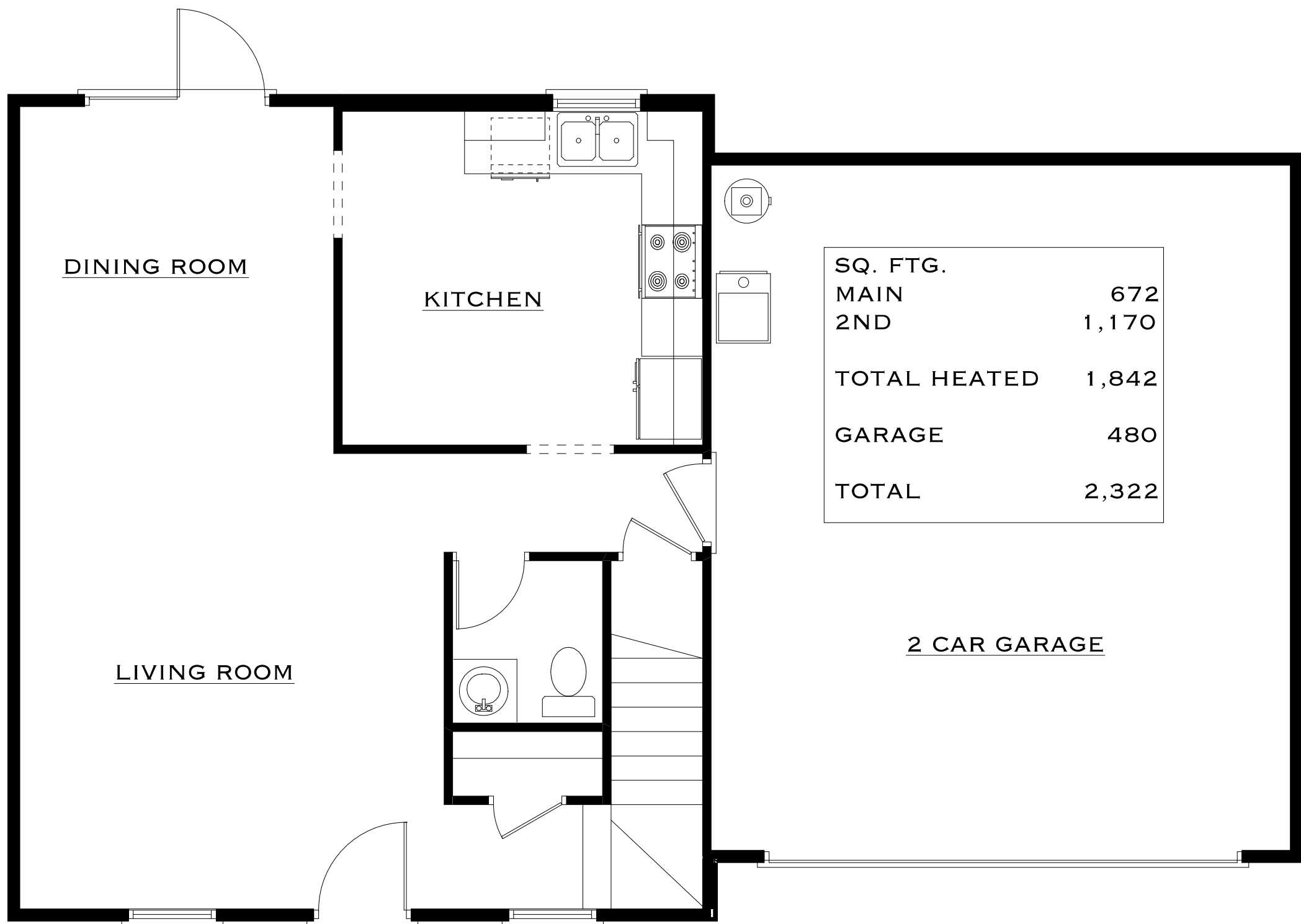
RUTHERFORD MODEL MAIN FLOOR PLAN
